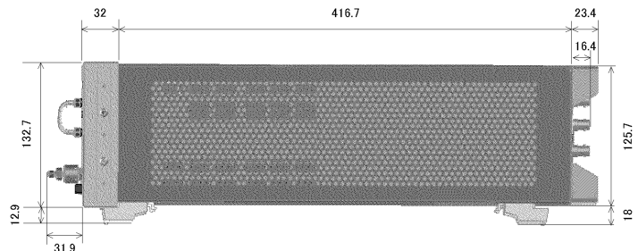
Figure 10-8. Side view
