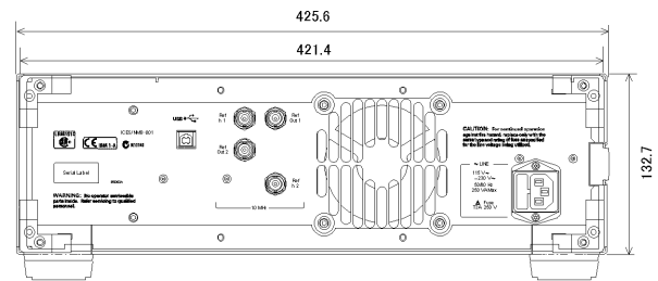
Figure 10-7. Rear view
