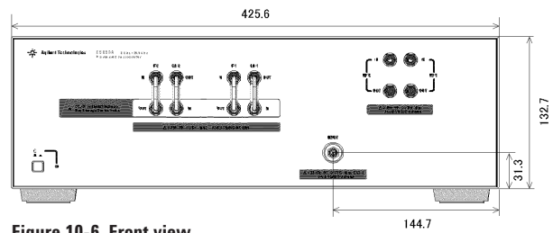
Figure 10-6. Front view
